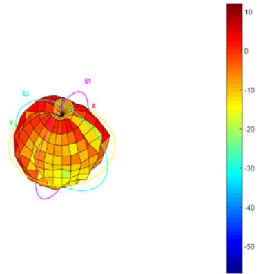
Total_3D_Side View 3_858MHz
