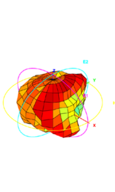
Total_3D_Side View 2_878MHz
