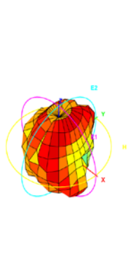
Total_3D_Side View 2_858MHz
