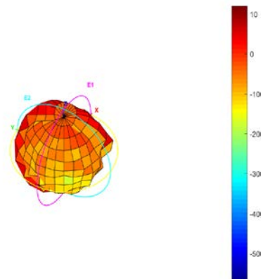
Total_3D_Side View 3_878MHz
