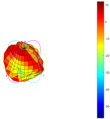
Total_3D_Side View 1_858MHz
