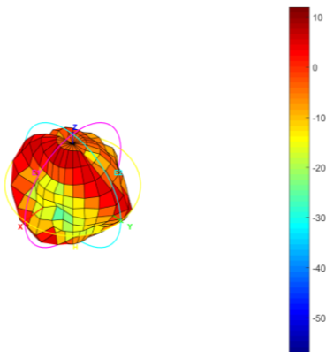
Total_3D_Side View 1_878MHz
