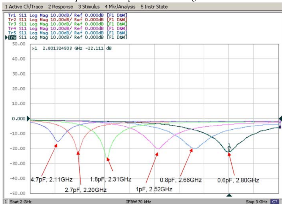
Frequencies VS. Capacitance Of Tuning Element
