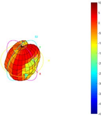
Total_3D_Side View 2_868MHz
