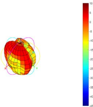
Total_3D_Side View 1_878MHz
