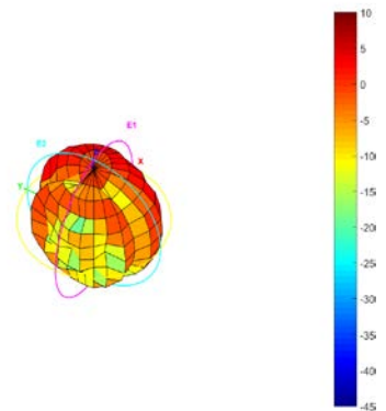
Total_3D_Side View 3_878MHz
