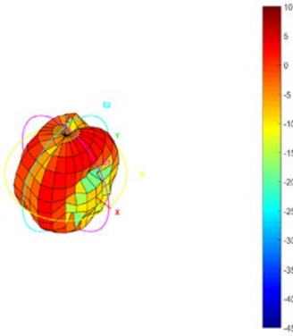
Total_3D_Side View 2_858MHz
