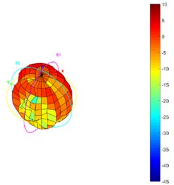
Total_3D_Side View 3_868MHz
