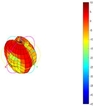
Total_3D_Side View 1_868MHz
